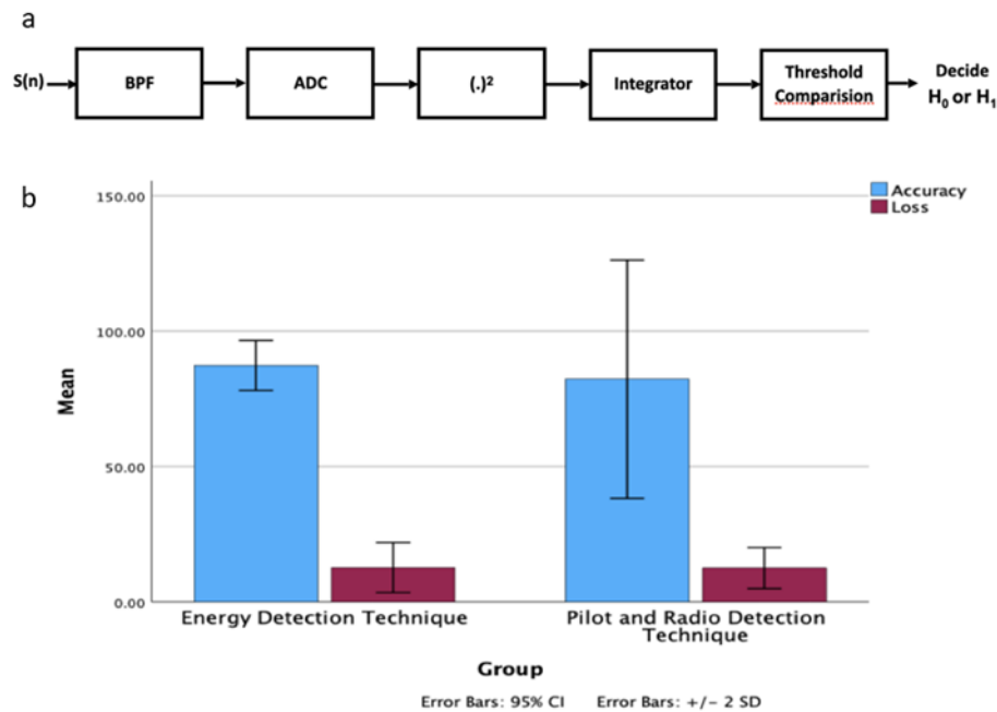
Figure 1. (a) Fundamental Block Diagram for Energy Detection (b) Comparison of Accuracy of Energy Detection Technique with Pilot and Radio Detection Technique in terms of mean Accuracy. The mean accuracy of the Energy Detection is higher than the Pilot and Radio Detection and the standard deviation of the Energy Detection is better than the Pilot and Radio Detection. Bar graph comparison of Pilot and Radio Detection which has mean accuracy of 93.9702% compared to Energy Detection which has mean accuracy of 95.2713%. X-axis algorithm, Y-axis mean accuracy with SD \pm 2 SD.
